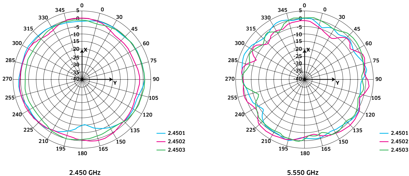
Figure 1. AP225 Antenna pattern plots: Horizontal or azimuth plane (top view)
