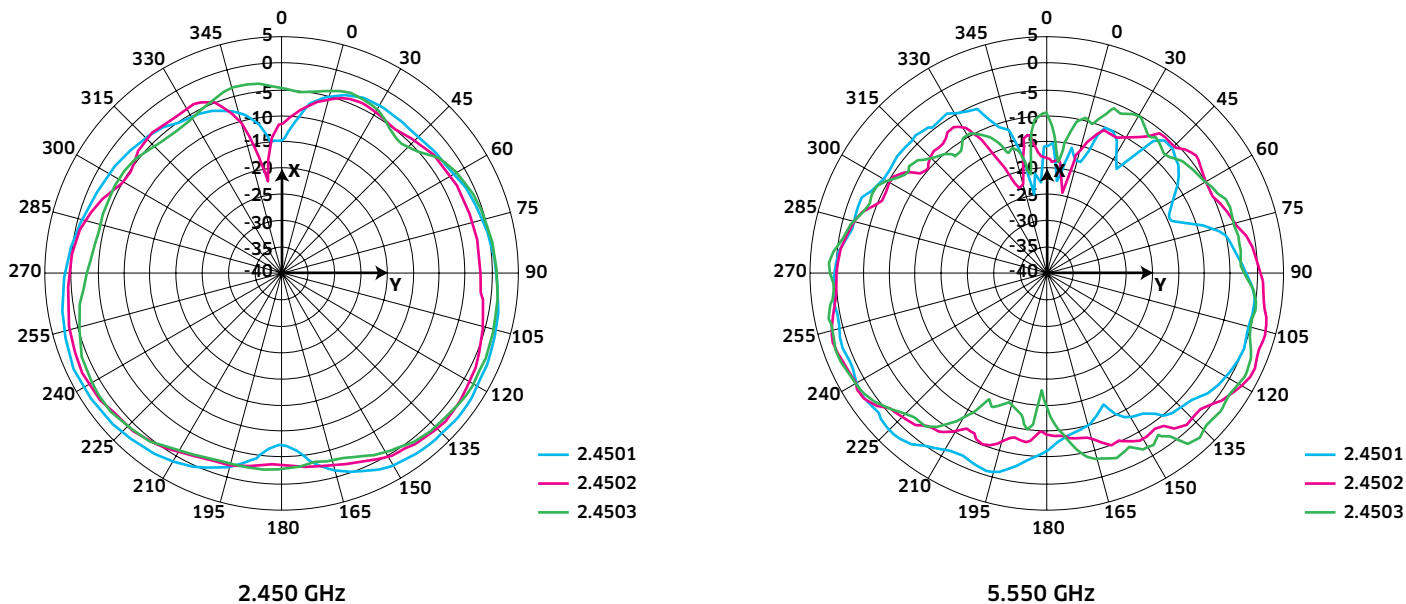
Figure 2. AP225 Antenna pattern plots: Elevation plane (side view)
